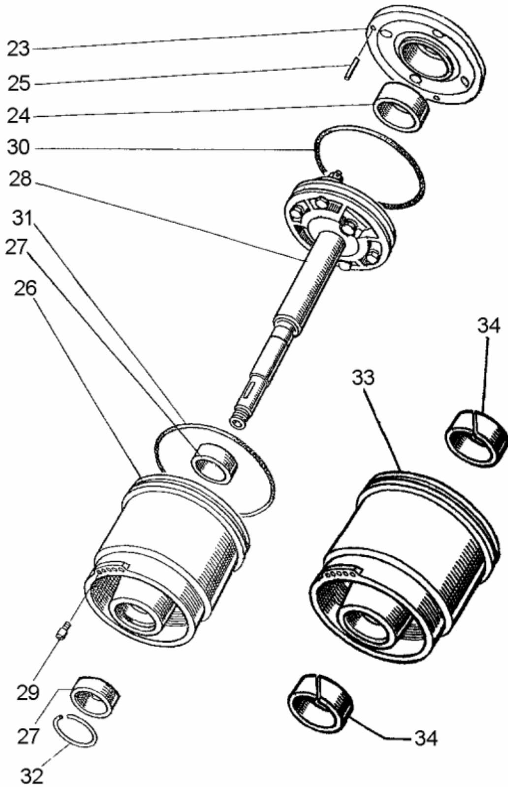
Fig. 9. Servo (Ctd.)
